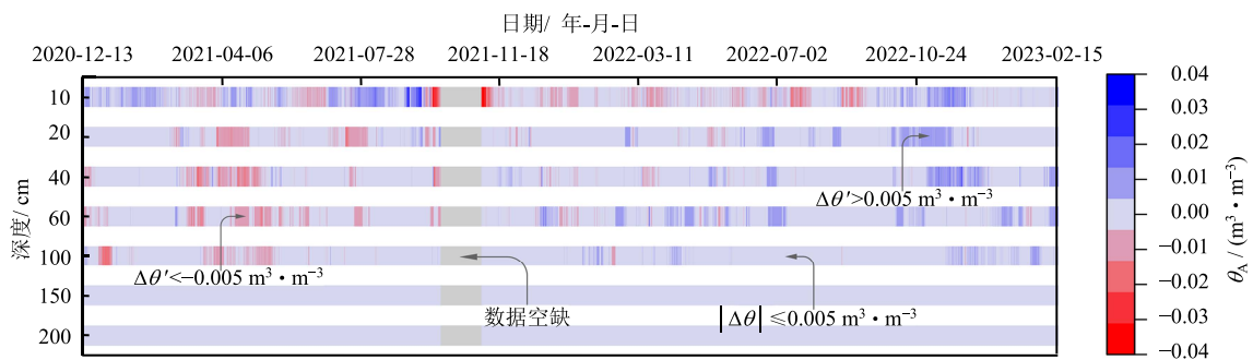
图7 含水率预测误差时空分布 Fig.7 Distribution of water content prediction errors
